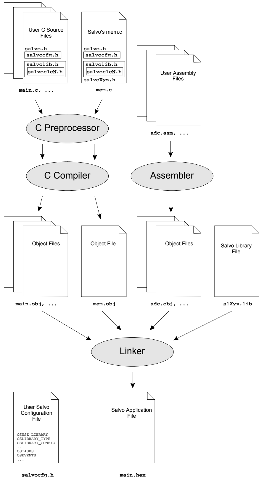
Figure 28: Salvo Library Build Overview
