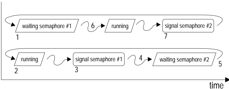
Figure 10: Synchronizing Two Tasks with Event Flags
